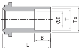
FR Gland to Short Tube Socket Weld
